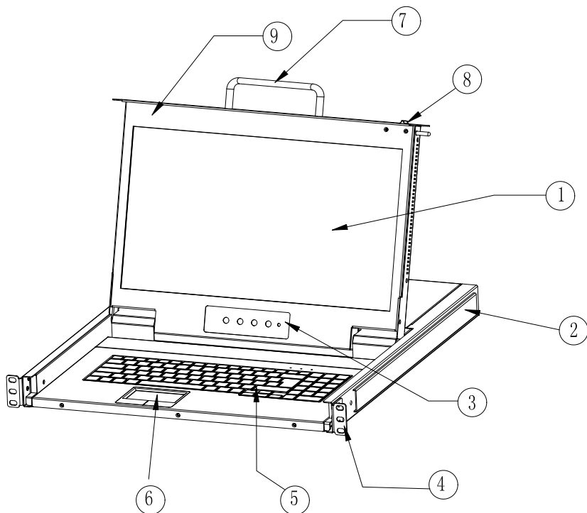
1-2 front view
